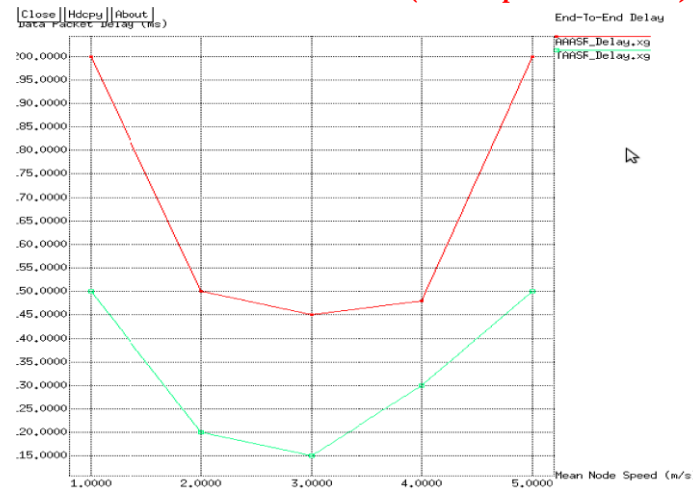
Figure 4: Comparison of TAASR Delay and AASR Delay
