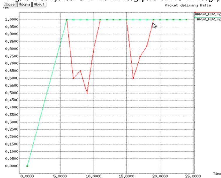
Figure 3: Comparison of TAASR PDR and AASR PDR
