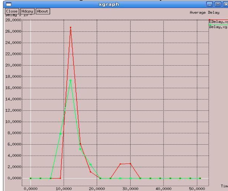
Figure 4: Delay Vs Time plot for FCFS and PB packet scheduling schemes
