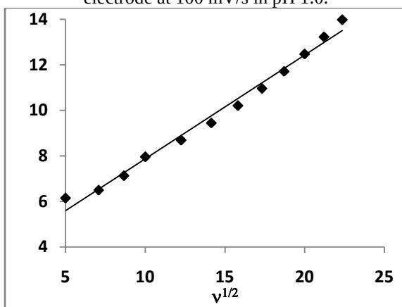
Figure 5: Plot of peak current vs square root of scan rate
